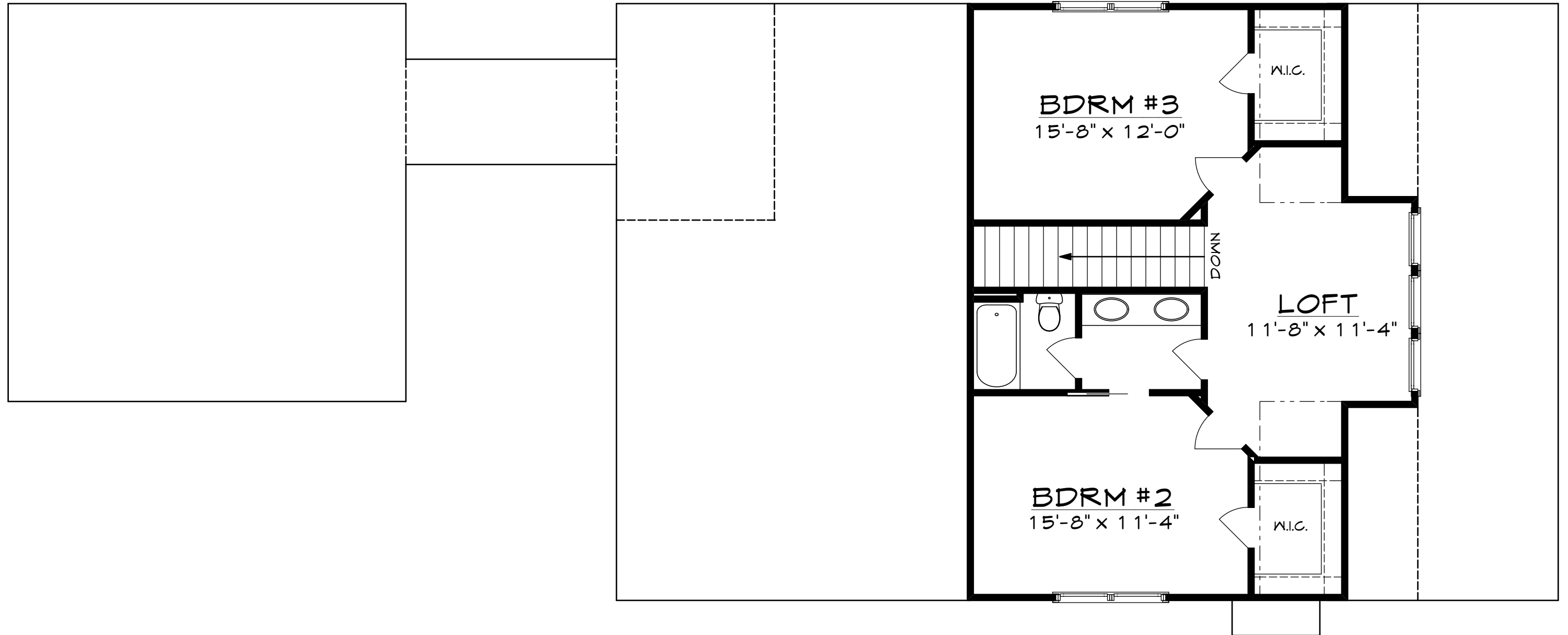
SECOND FLOOR PLAN 726 SF HTD.
