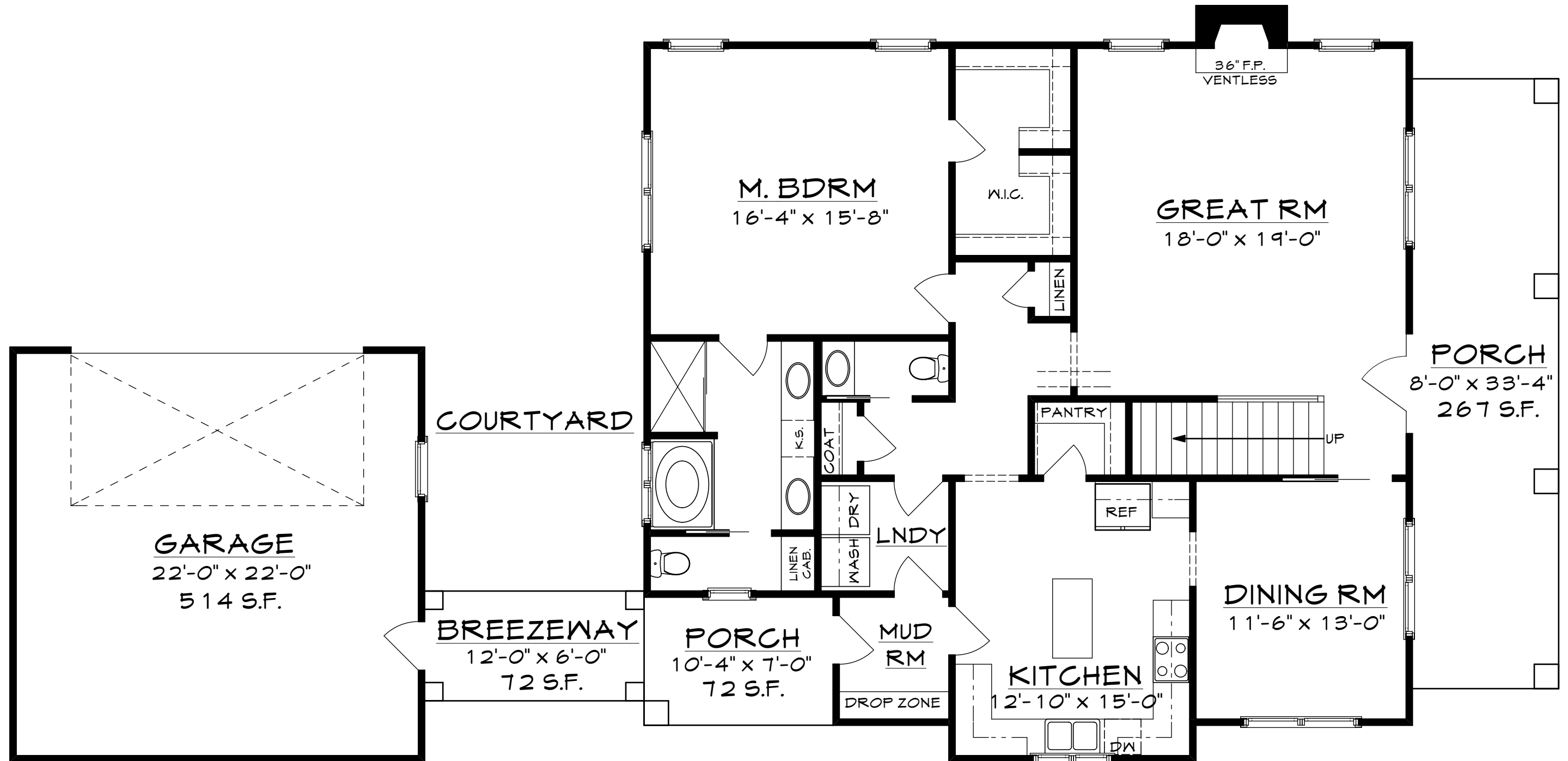
FIRST FLOOR PLAN 1522 SF HTD.
